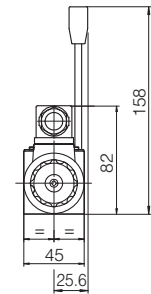
DHE-06*/MV Mass: 2,7 kg (single solenoid) DHE-07*/MV (dotted line) Mass: 3,0 kg (double solenoid)
