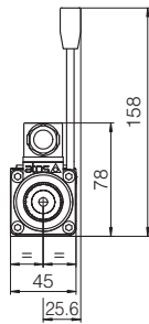
DHI-06*/MV Mass: 2,4 kg (single solenoid) DHI-07*/MV (dotted line) Mass: 2,7 kg (double solenoid)
