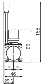
DHZO-A-05*/MV Mass: 2,8 kg (single solenoid) DHZO-A-07*/MV (dotted line) Mass: 3,5 kg (double solenoid)
